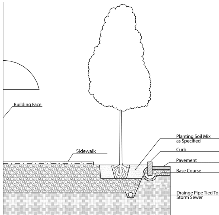
22 Planting Detail for Tree Wells 23 24 25
